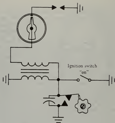
FIGURE 4-13. Typical ignition switch in the "on" position.
